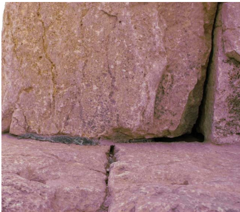
Fig. 2 Achaemenid Used the Lead as Mortars for Connecting Rock Fragments. Place: Tomb of Minor Cyrus, Bozpar
