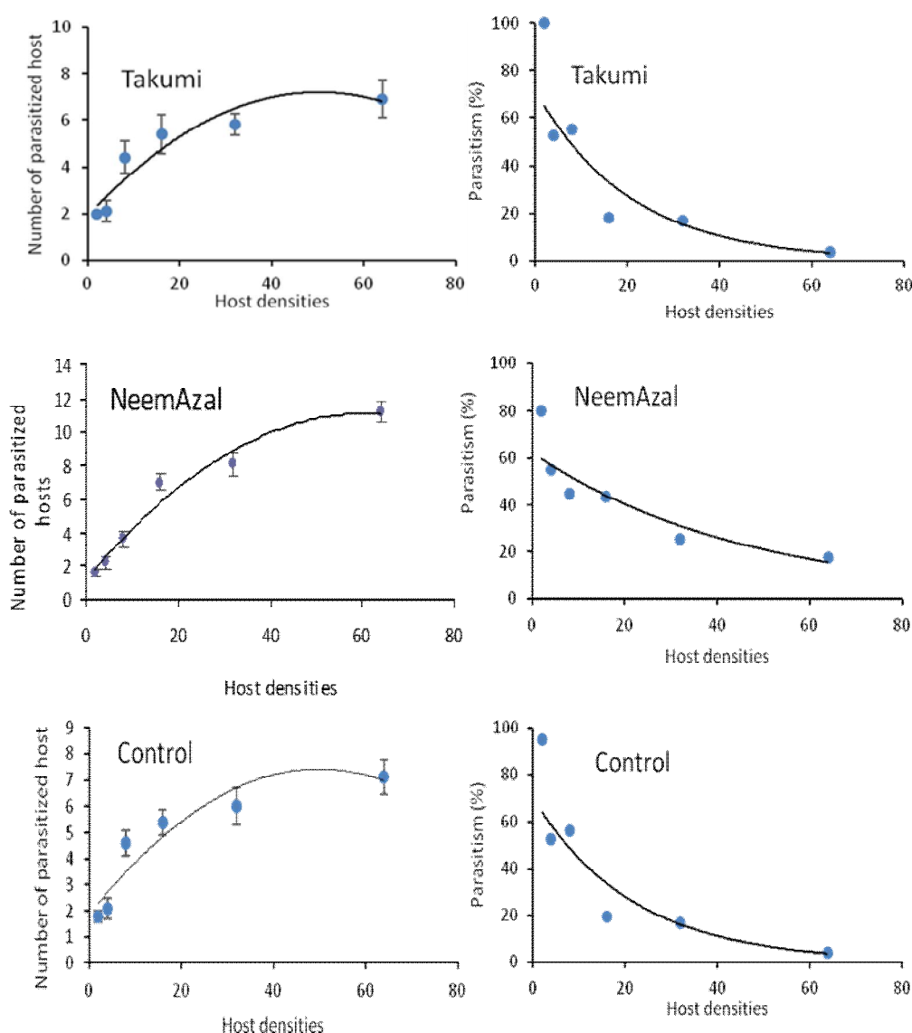
Figure 1 Functional response of the ectoparasitoid Habrobracon hebetor , exposed to field concentrations of Takumi and NeemAzal, and in the control.
