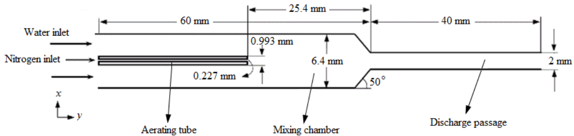
Fig. 1 Dimensions and various parts of the simulated atomizer
