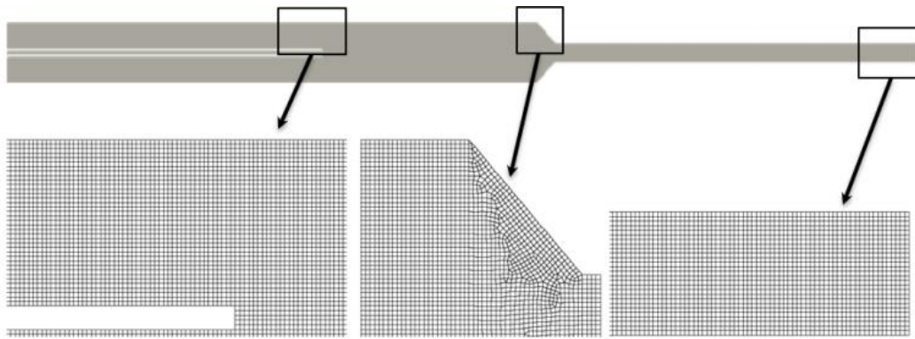
Fig. 2 Meshing strategy at different parts of the effervescent atomizer
