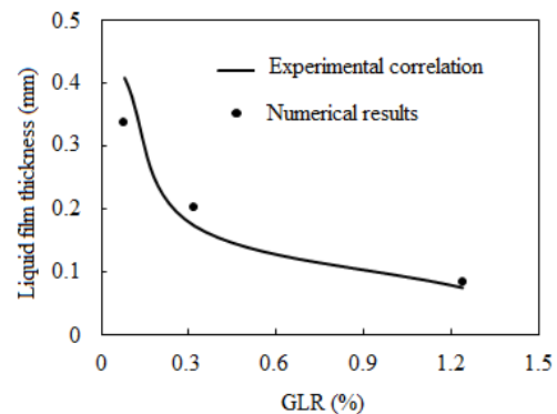
Fig. 4 The liquid film thickness of computed results in different aerating gas flow rates compare with measured thickness by Lin et al. [19]
