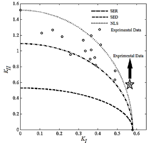
Fig. 3 Fracture limit curves for mixed mode loading of Norway spruce wood in comparison with experimental data[6]
